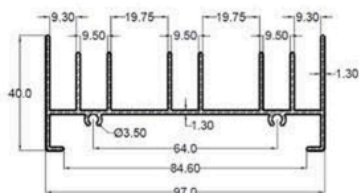
100-01 THREE HEAD
