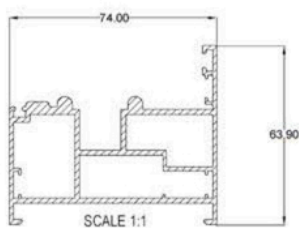
75-01 PERIMETER
