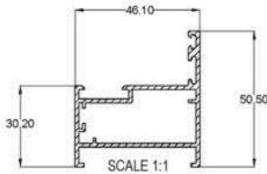
A69-01A PERIMETER
