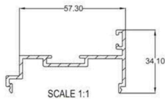
75-04 PANEL ASTRAGAL
