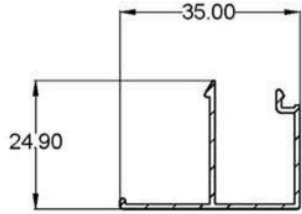
85-35 MM MOULDING
