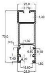
100-07 PANEL
