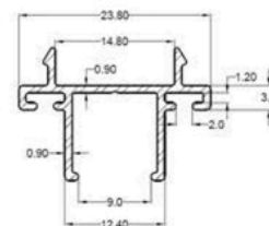
100-13 PANEL ASTRAGAL
