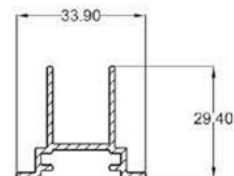
75-05 DRIVE GROOVE
