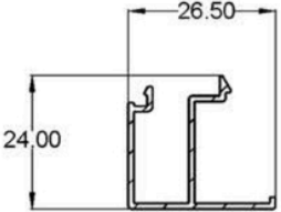
60-68 27MM MOULDING
