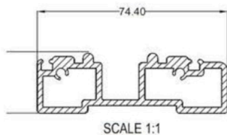
75-02 PERIMETER
