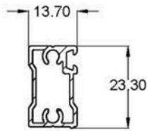
85-04 WINDOW GRILL
