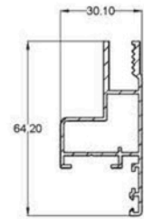
30-65 SCREEN PANEL
