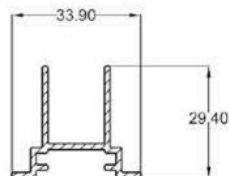
75-05 DRIVE GROOVE
