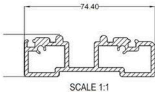
75-02 PERIMETER
