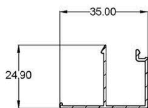
85-35 MM MOULDING
