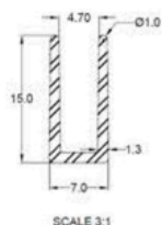
100-22 SECURITY SCREEN MOULDING
