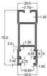
100-07 PANEL
