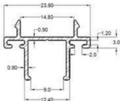
100-13 PANEL ASTRAGAL
