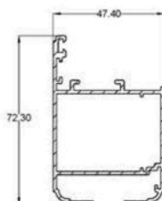
A68-03 WINDOW PANEL
