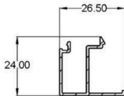
60-68 27MM MOULDING
