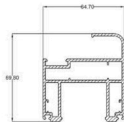
75-03 PANEL
