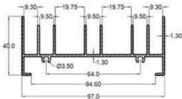
100-01 THREE HEAD
