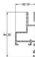
30-65 SCREEN PANEL
