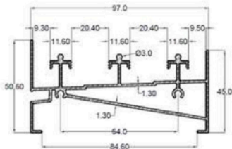
100-02 THREE SILL
