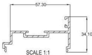
75-04 PANEL ASTRAGAL
