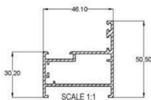
A69-01A PERIMETER
